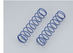
No.IF348-1016 Big Shock Spring (M&L/Blue/10-1.6/L=95)
